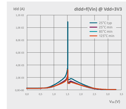
LVT input curves at 3V3
