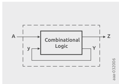
Figure 4.1 | Asynchronous Logic element
