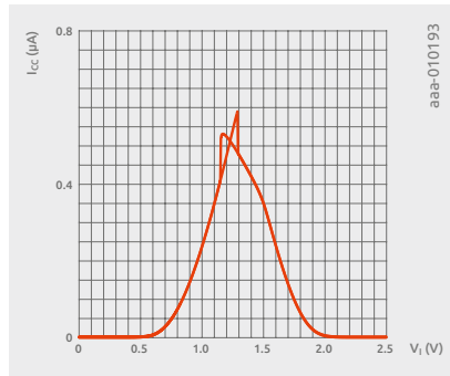
2.5 V Schmitt action
