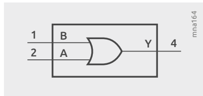
Figure 2.4a | IEEE symbol of an OR gate
