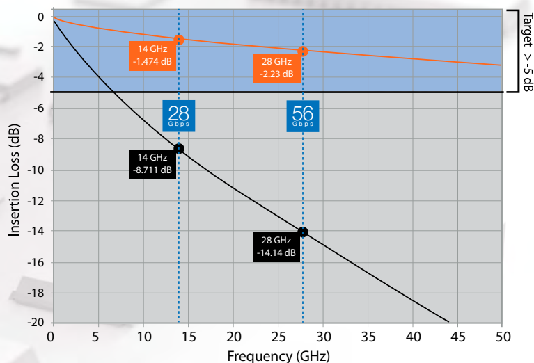
Ultra Low Skew Twinax vs. PCB Traces
